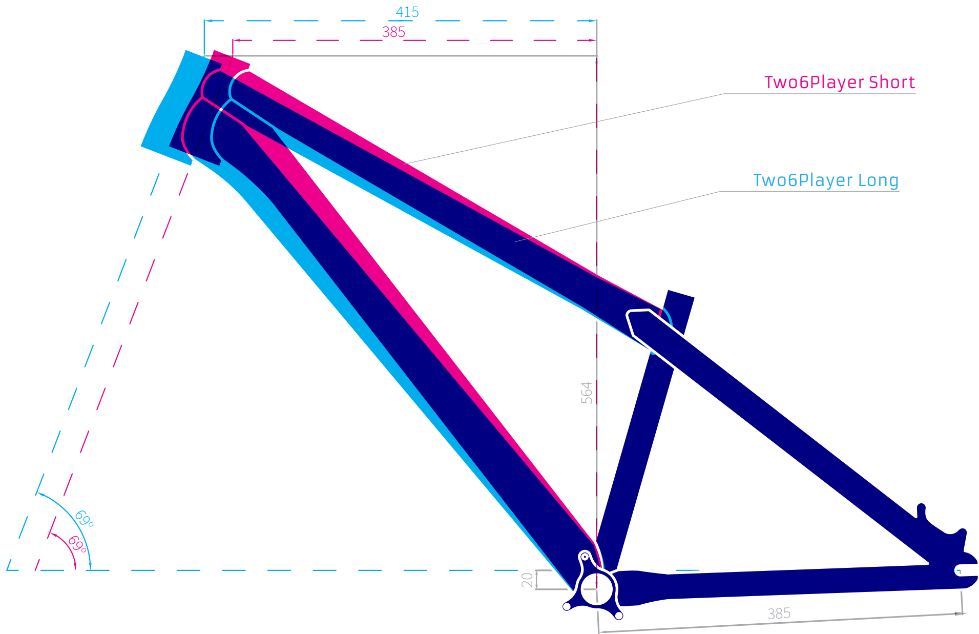
GEOMETRY OF DARTMOOR TWO6PLAYER FRAME SIZES
